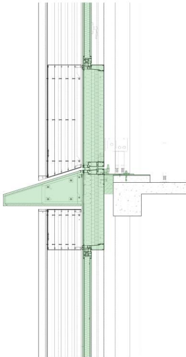
EWS - 101 Floor Edge Detail (Opaque Panel)
