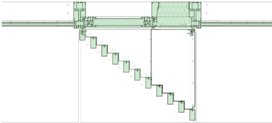
EWS - 101 Typical Mullion Detail
