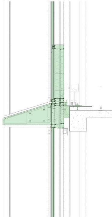
EWS - 101 Floor Edge Detail (Vision Panel)
