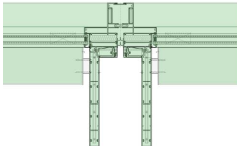
EES-10 - Typical mullion (right)
