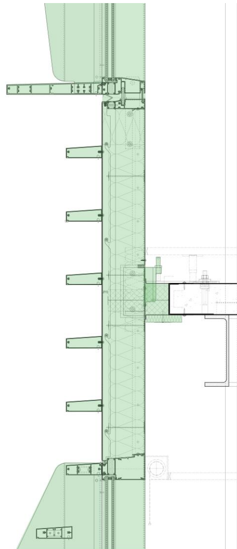
EES-10 - Typical floor edge detail
