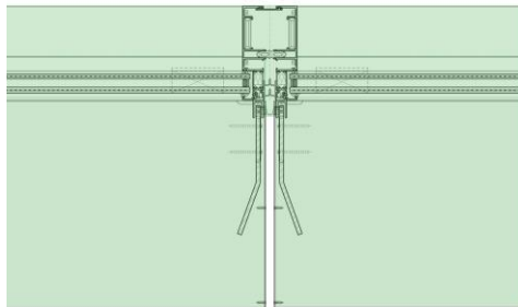
EES-10 - Typical mullion (left)
