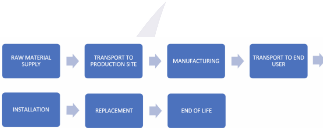
Figure: LCA process diagram according to EN 15804 (7.2.1)
